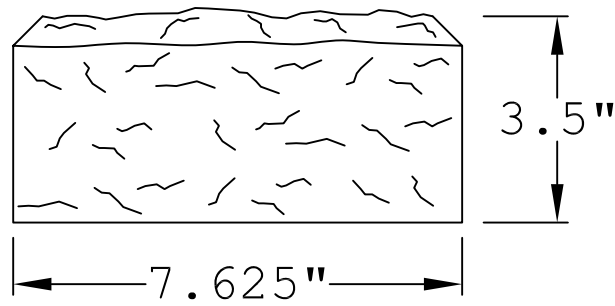
SIDE/END VIEW
