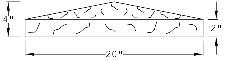
END VIEW
