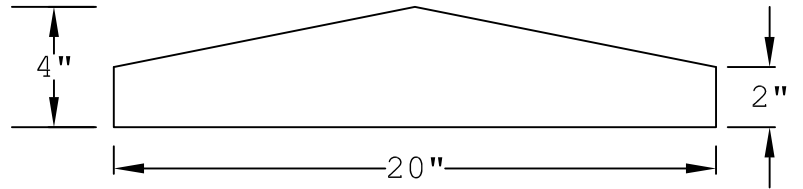
END VIEW
