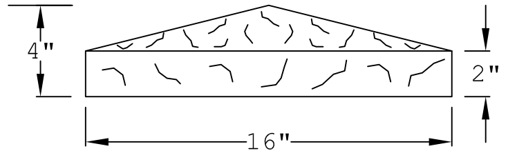
END VIEW
